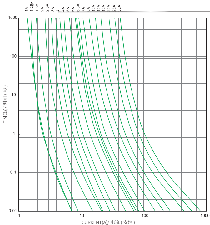
65TS AVERAGE I-T CHARACTERISTICS CURVE (FOR REFERENCE ONLY) 65TS I-T ( )
